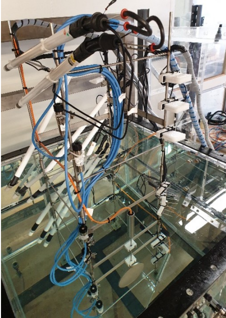
Figure 3. Instrumentation on internal mounting frame.
