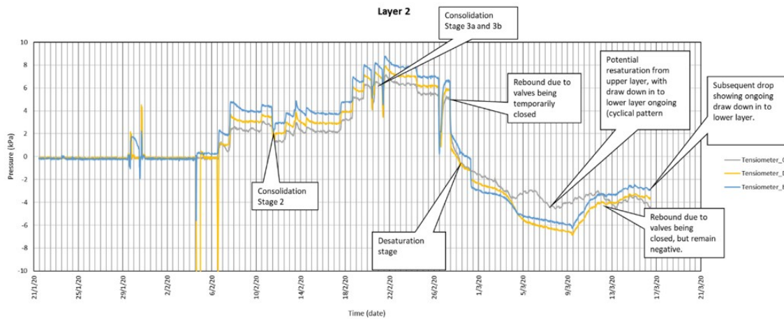
Figure 5. Suction pressures developed in tailings layer 2.
